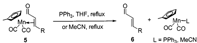
Scheme 5. Demetalation of the \alpha,\beta -unsaturated aldehydes 6
